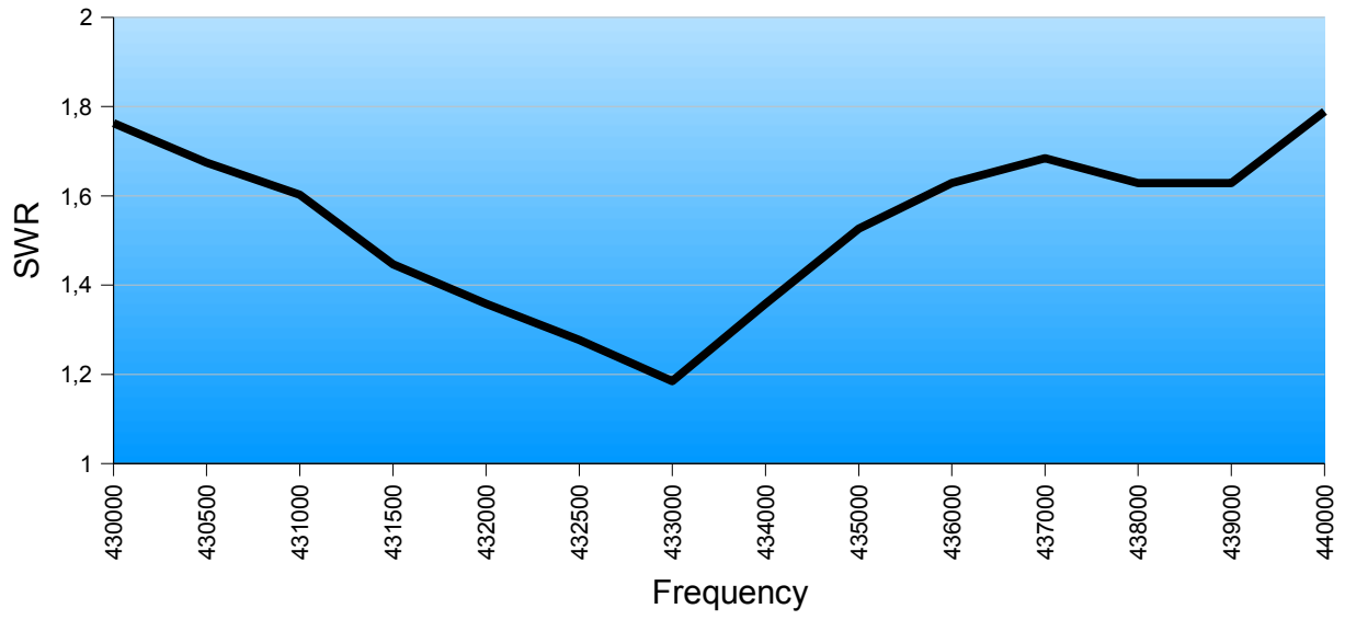
70cm SWR Chart ON3JT
