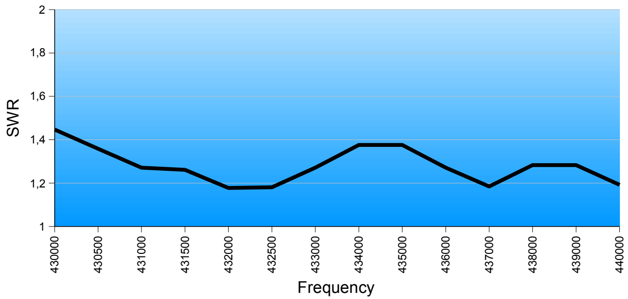
70cm SWR Chart ON5NV
