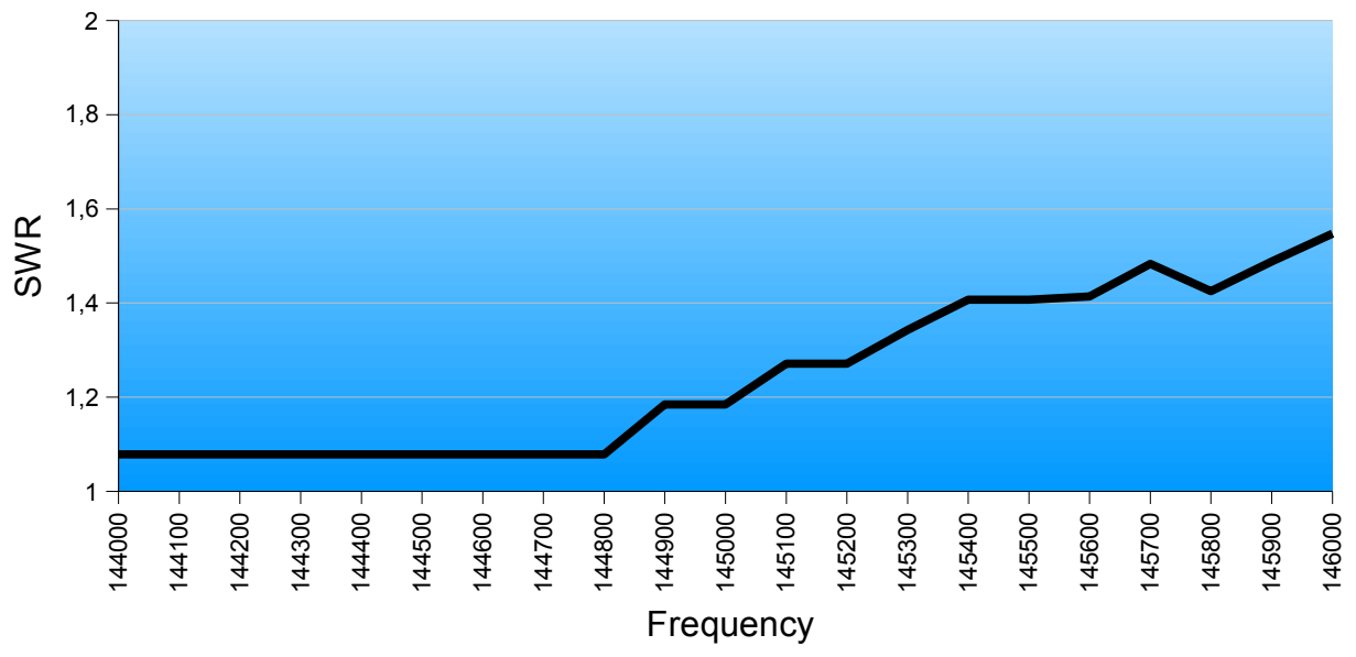
2 meter SWR Chart ON5NV
